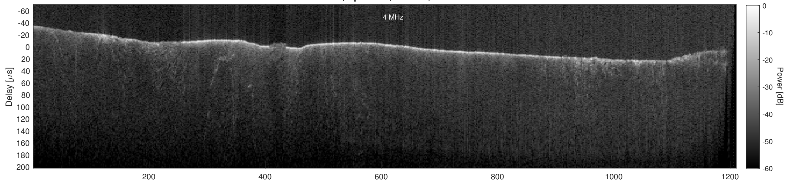
Orbit 10068, Cluttergram
