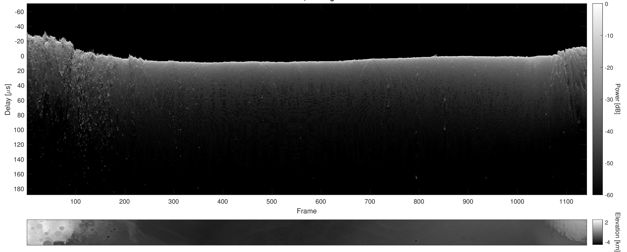
Orbit 10069, Cluttergram
