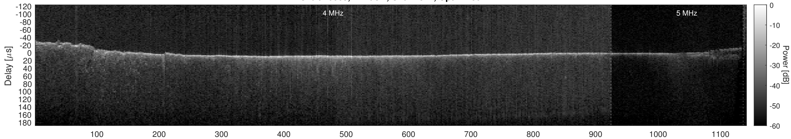
Orbit 10069, Cluttergram
