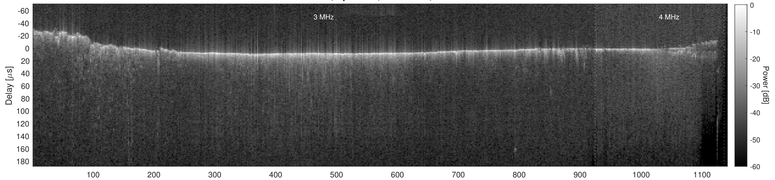
Orbit 10069, Cluttergram
