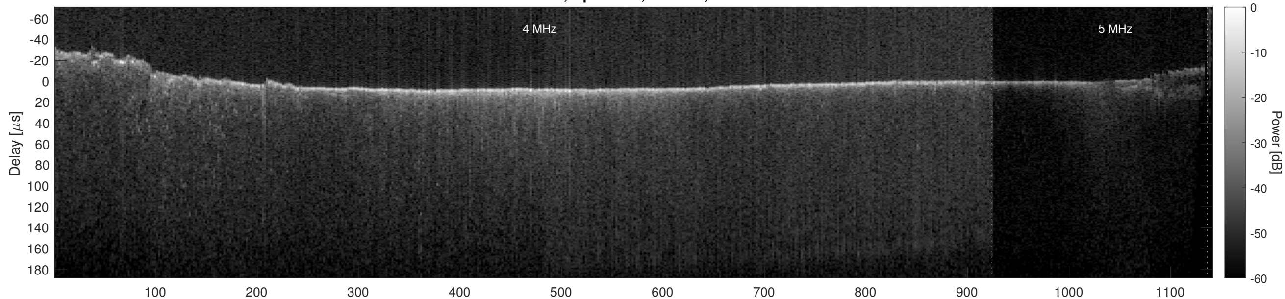
Orbit 10069, Optimized, Window, Channel 2
