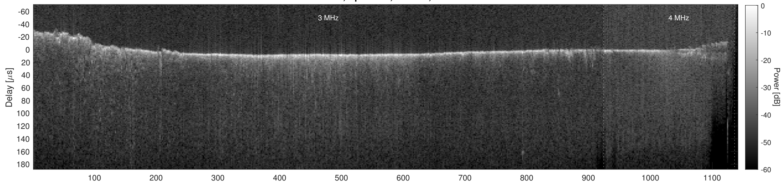
Orbit 10069, Cluttergram
