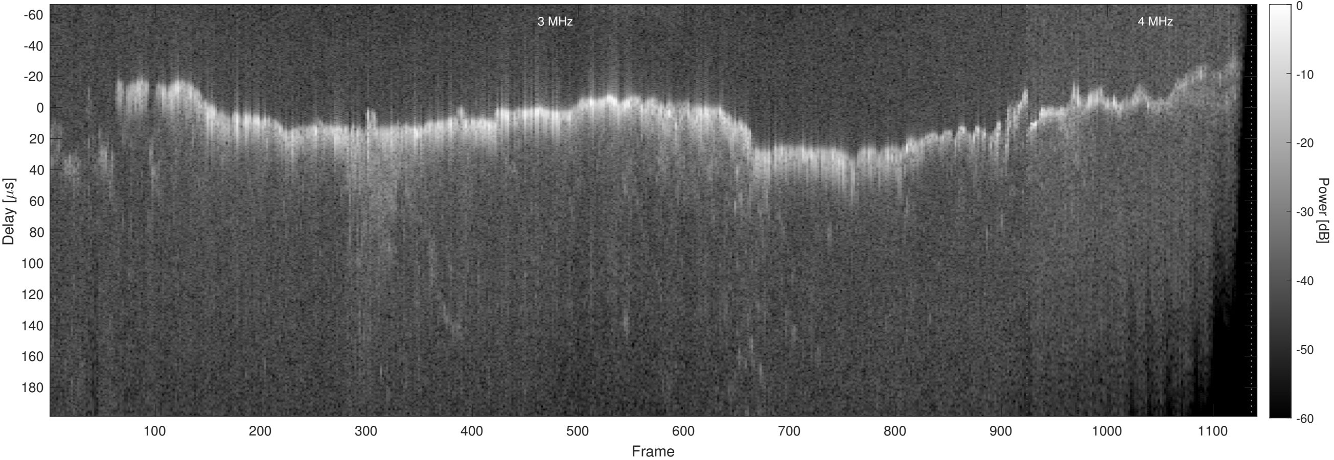
Orbit 10071, Chapman, No Window, Channel 2
