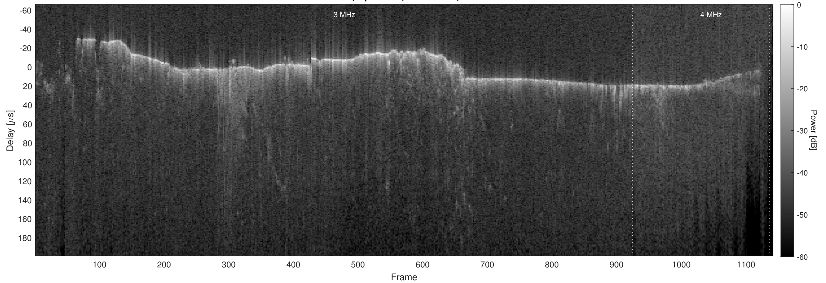
Orbit 10071, Optimized, No Window, Channel 2
