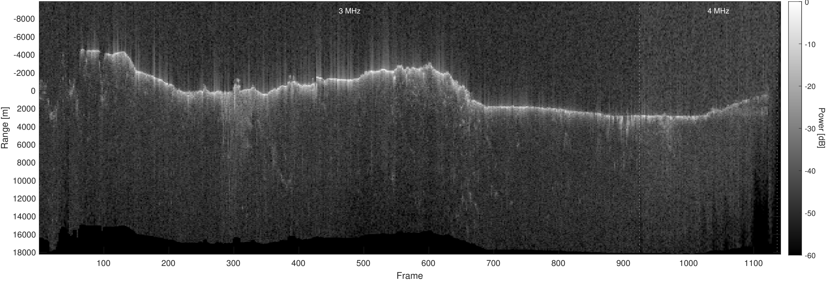
Orbit 10071, Optimized, No Window, Depth-Corrected, Channel 2
