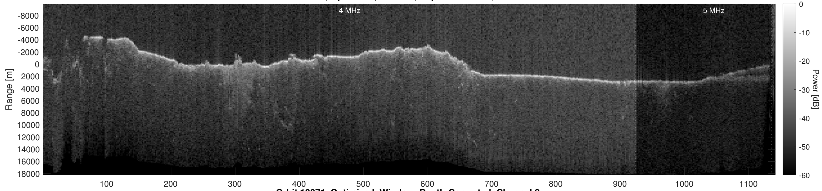
Orbit 10071, Optimized, Window, Depth-Corrected, Channel 2
