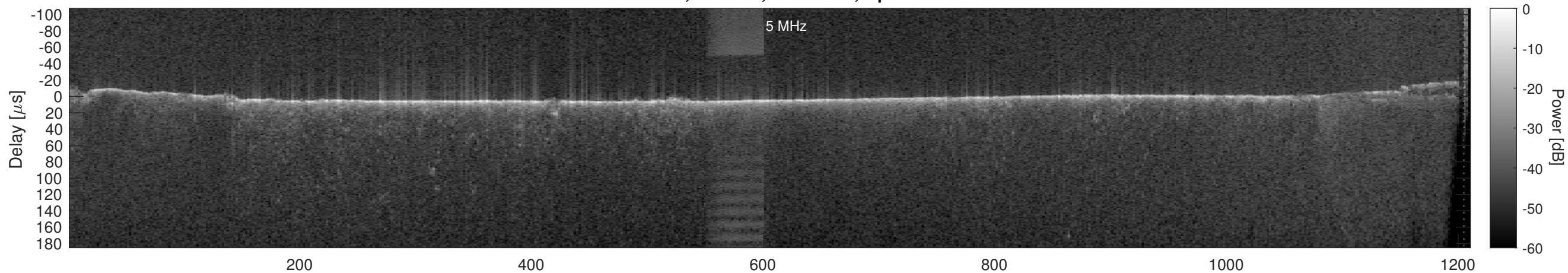
Orbit 10072, Cluttergram
