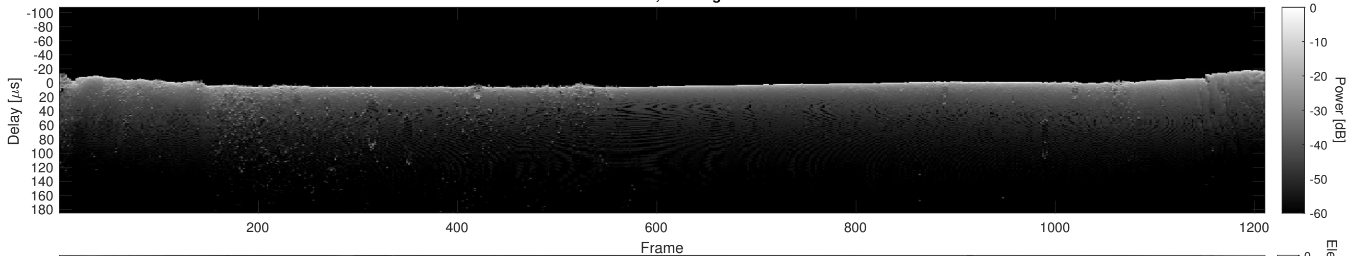
Orbit 10072, Cluttergram
