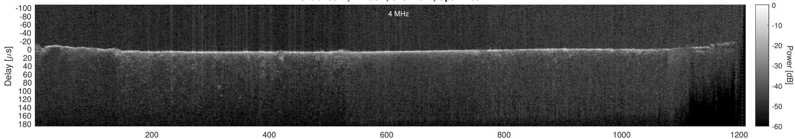
Orbit 10072, Cluttergram
