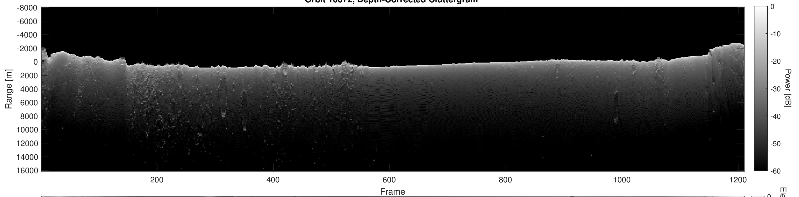
Orbit 10072, Depth-Corrected Cluttergram
