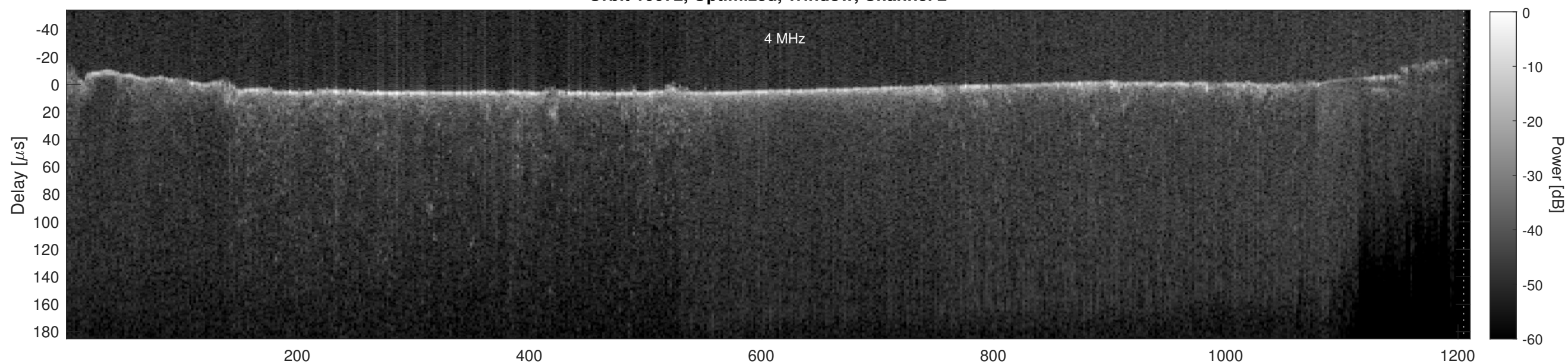
Orbit 10072, Cluttergram
