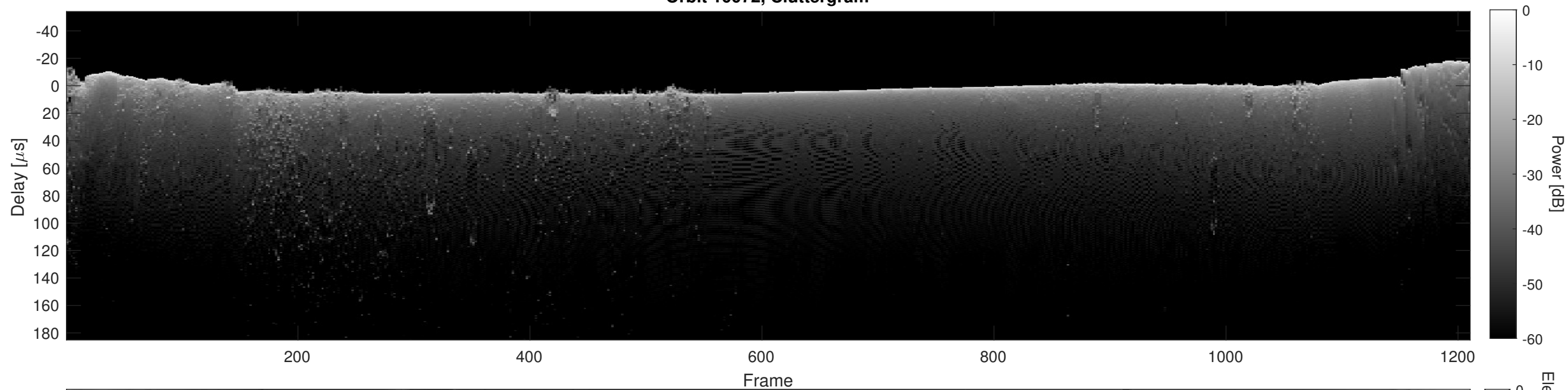
Orbit 10072, Cluttergram
