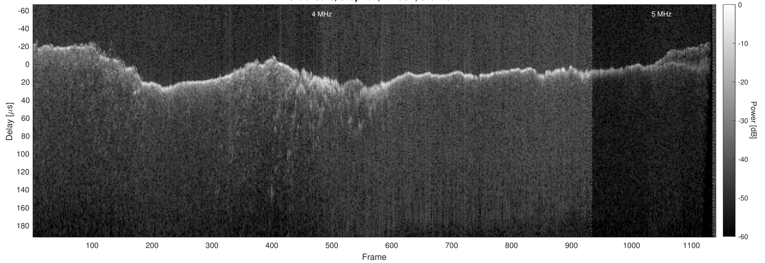
Orbit 10073, Chapman, Window, Channel 2
