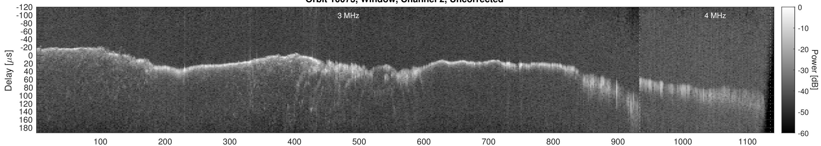
Orbit 10073, Window, Channel 2, Chapman
