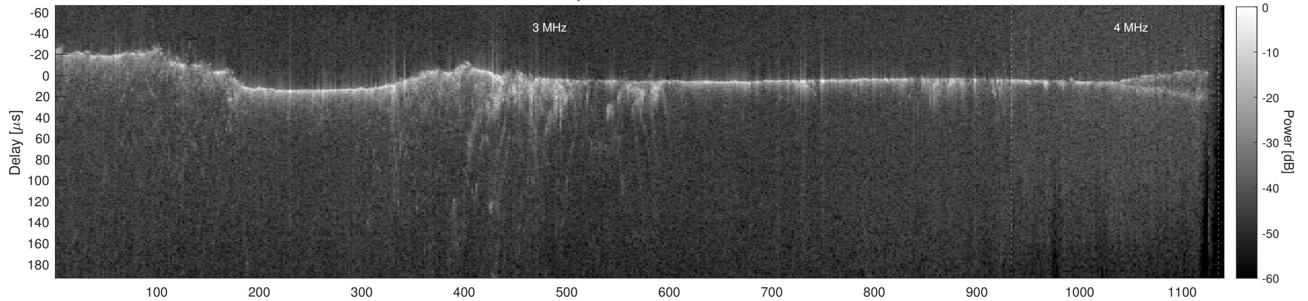
Orbit 10073, Cluttergram
