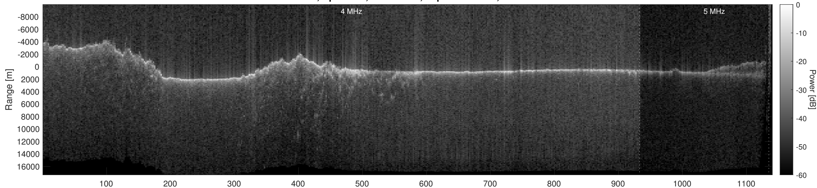
Orbit 10073, Optimized, No Window, Depth-Corrected, Channel 2
