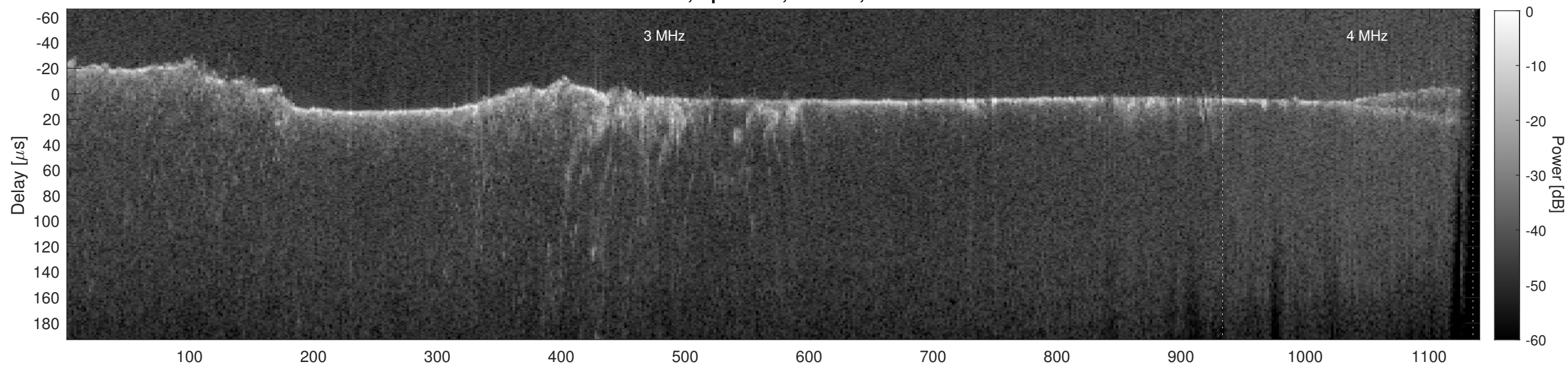
Orbit 10073, Cluttergram
