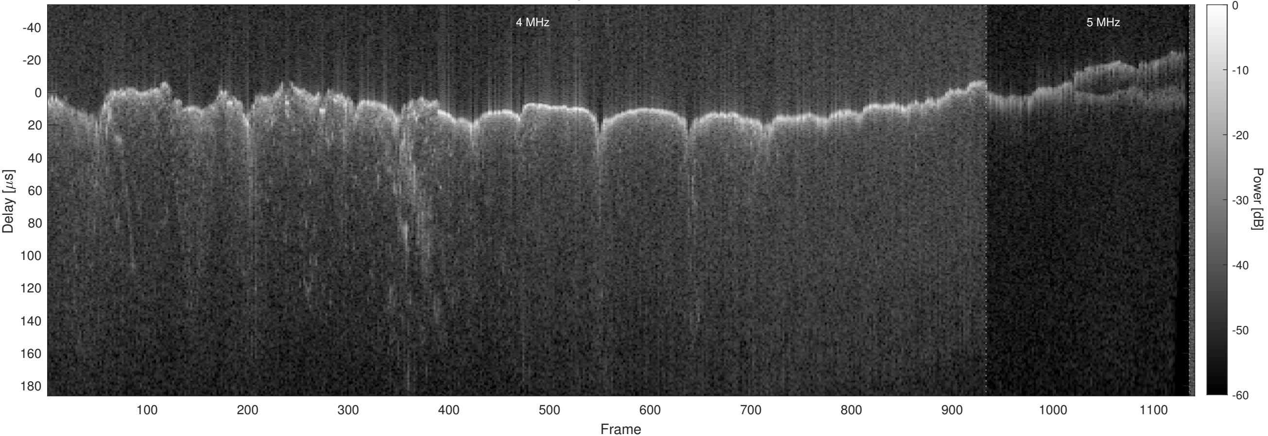
Orbit 10074, Chapman, No Window, Channel 2
