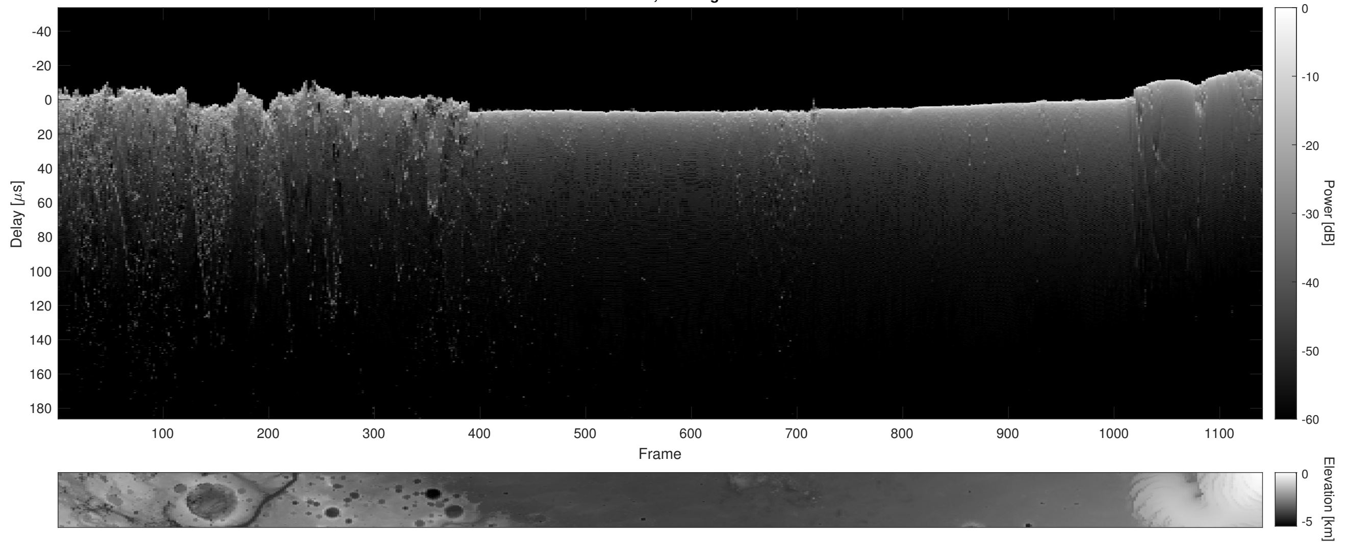
Orbit 10074, Cluttergram
