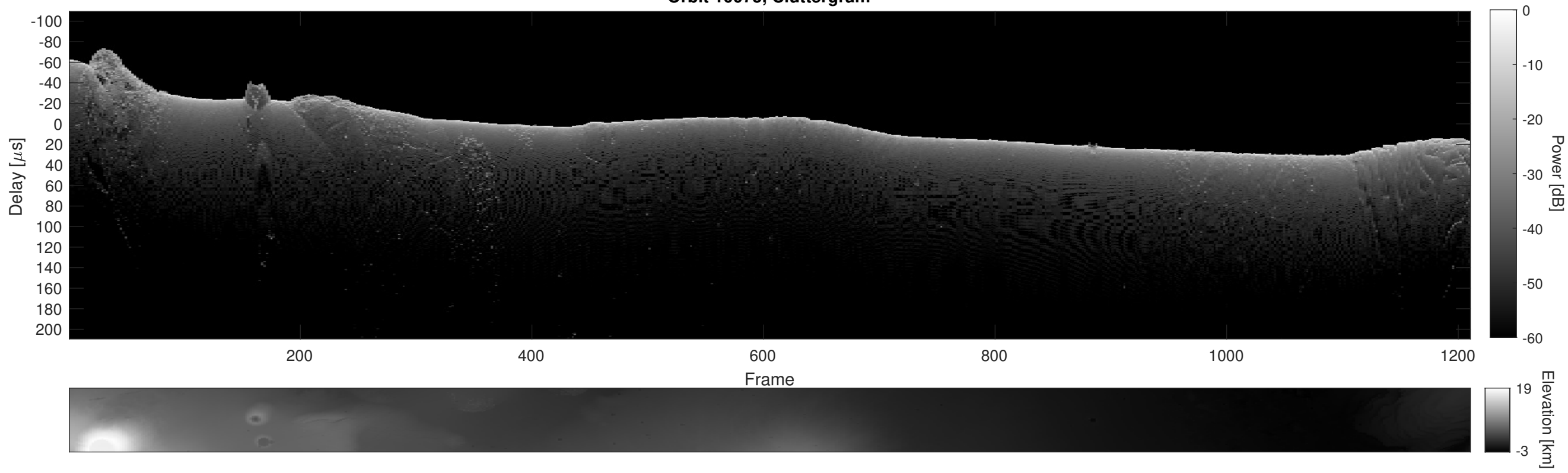
Orbit 10075, Cluttergram
