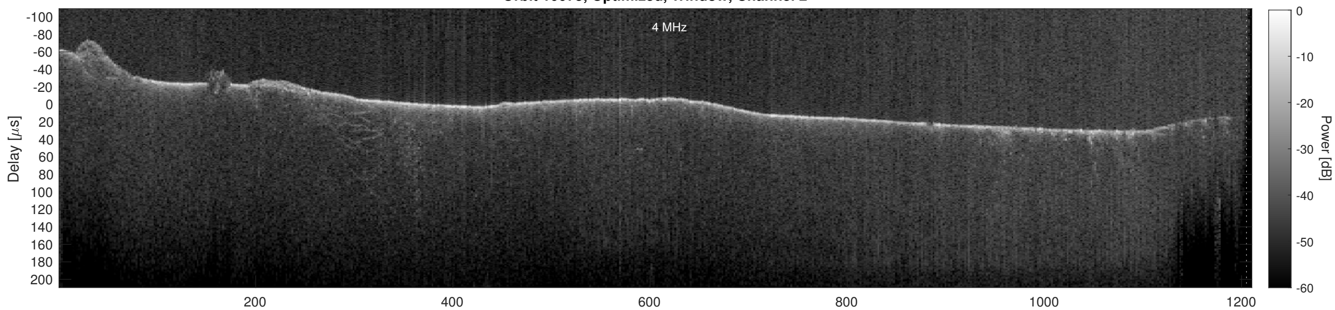
Orbit 10075, Cluttergram
