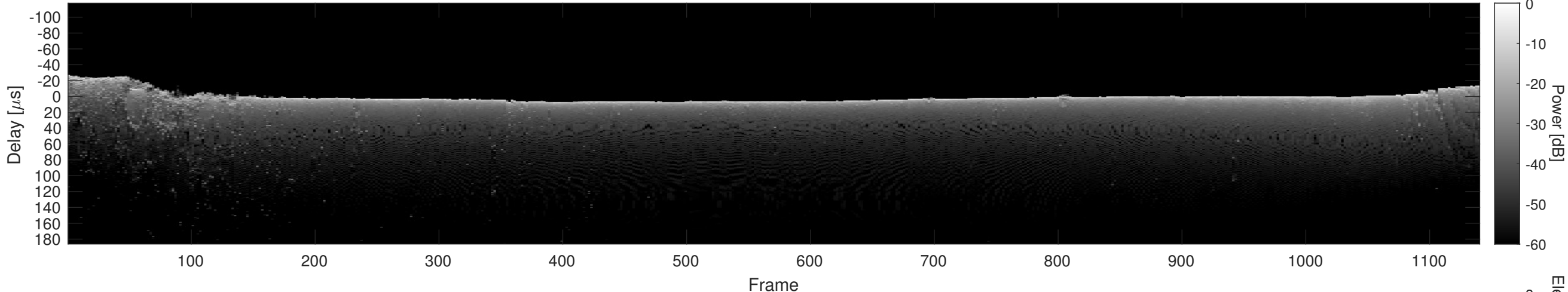
Orbit 10076, Cluttergram
