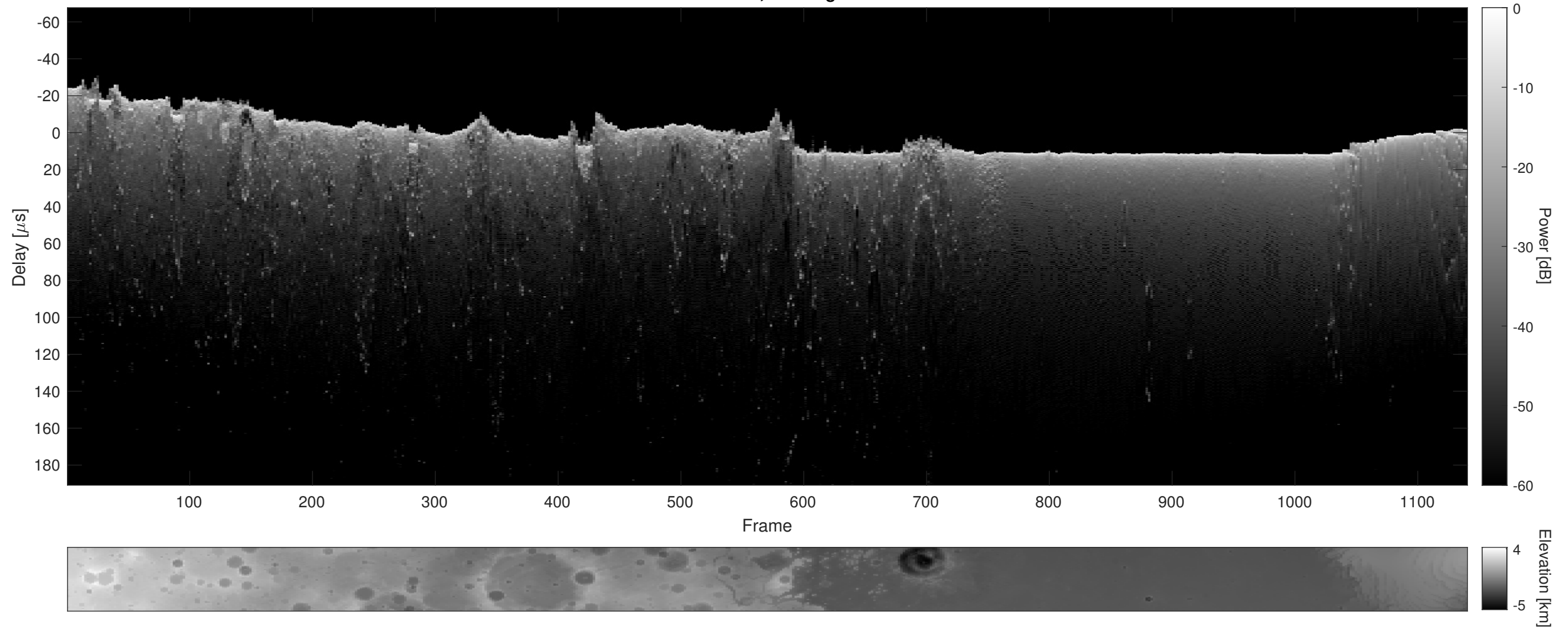
Orbit 10077, Cluttergram
