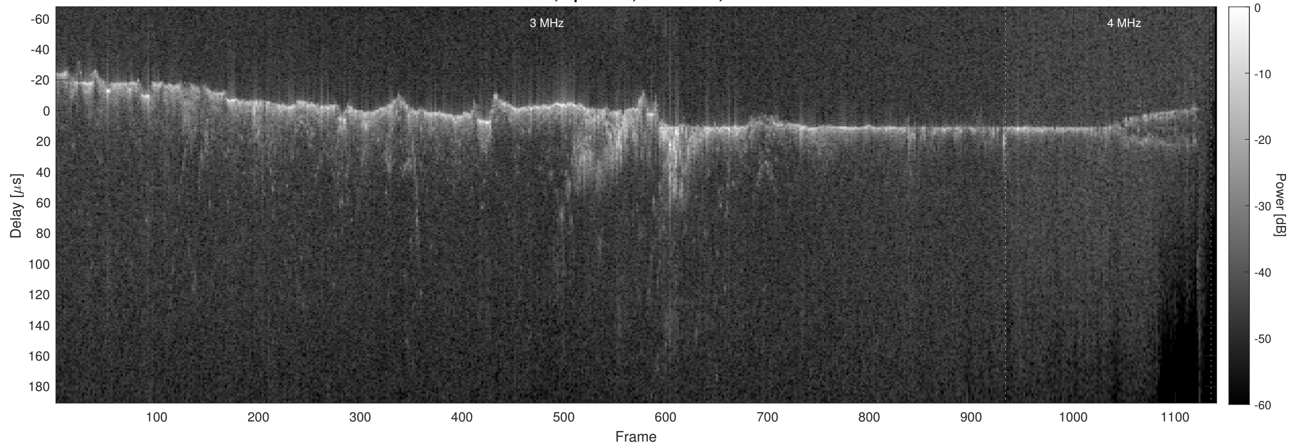
Orbit 10077, Optimized, No Window, Channel 2
