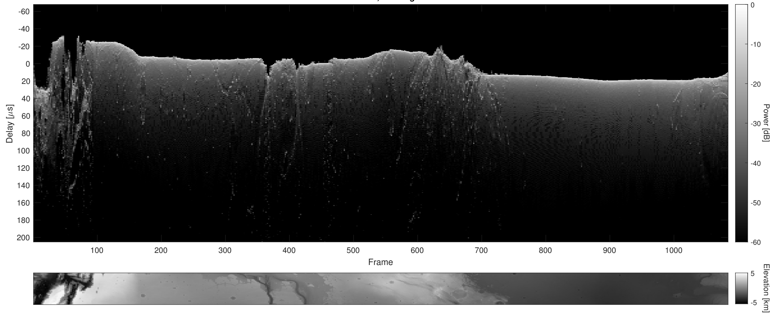
Orbit 10078, Cluttergram
