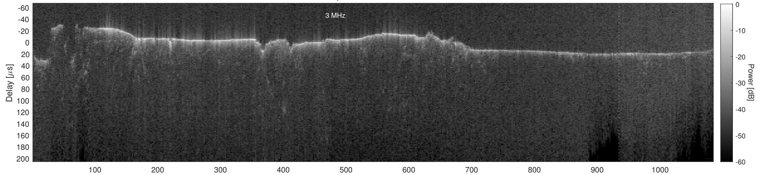
Orbit 10078, Cluttergram
