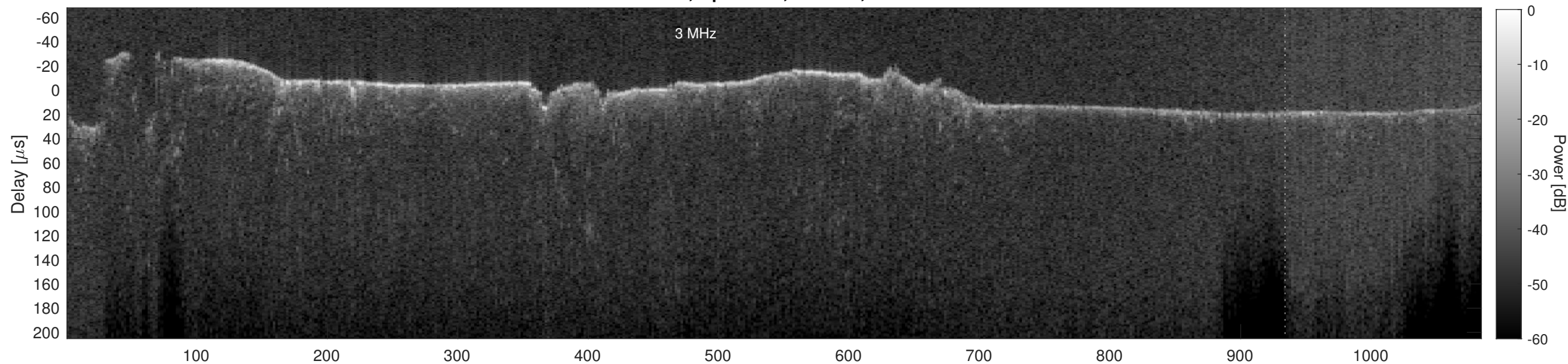
Orbit 10078, Cluttergram
