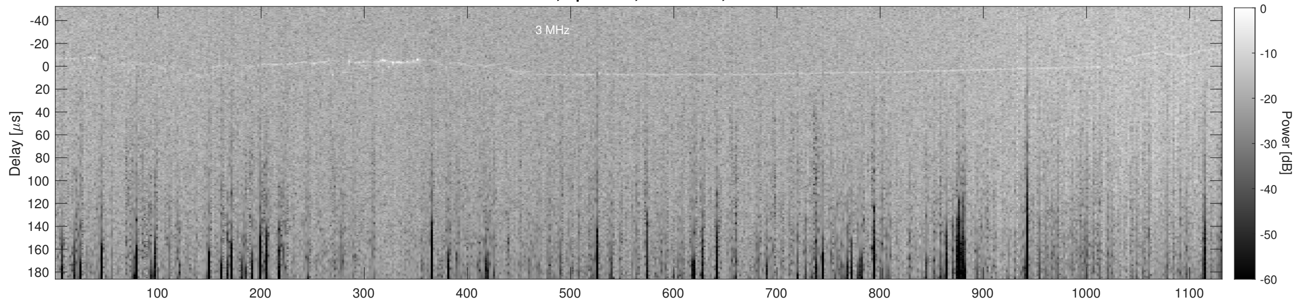
Orbit 10081, Cluttergram
