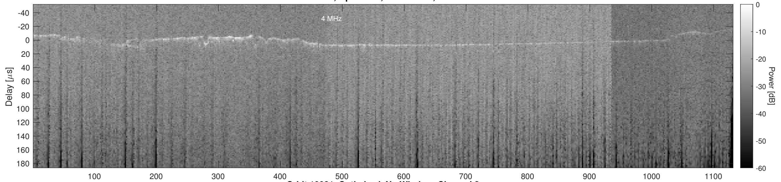
Orbit 10081, Optimized, No Window, Channel 2
