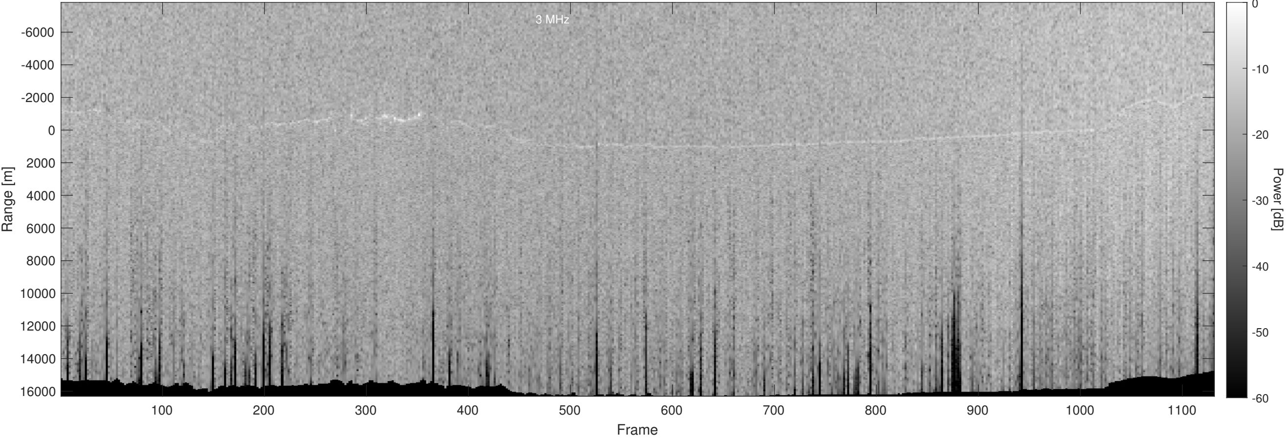
Orbit 10081, Optimized, No Window, Depth-Corrected, Channel 2
