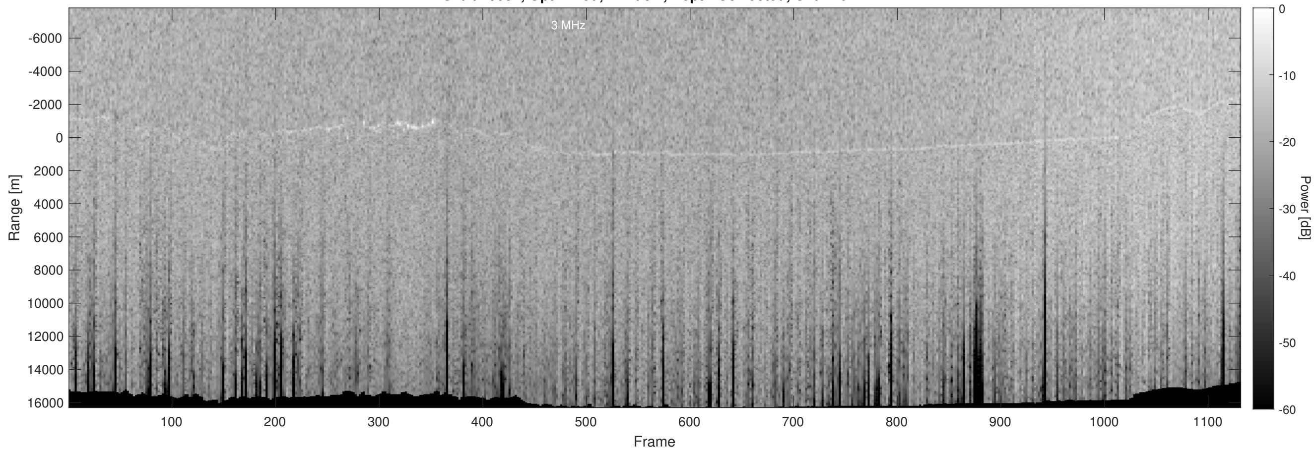
Orbit 10081, Optimized, Window, Depth-Corrected, Channel 2
