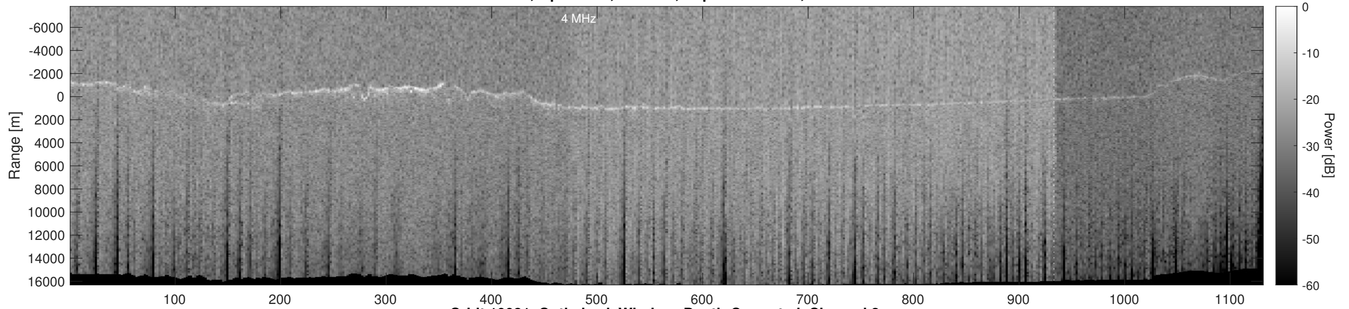
Orbit 10081, Optimized, Window, Depth-Corrected, Channel 2
