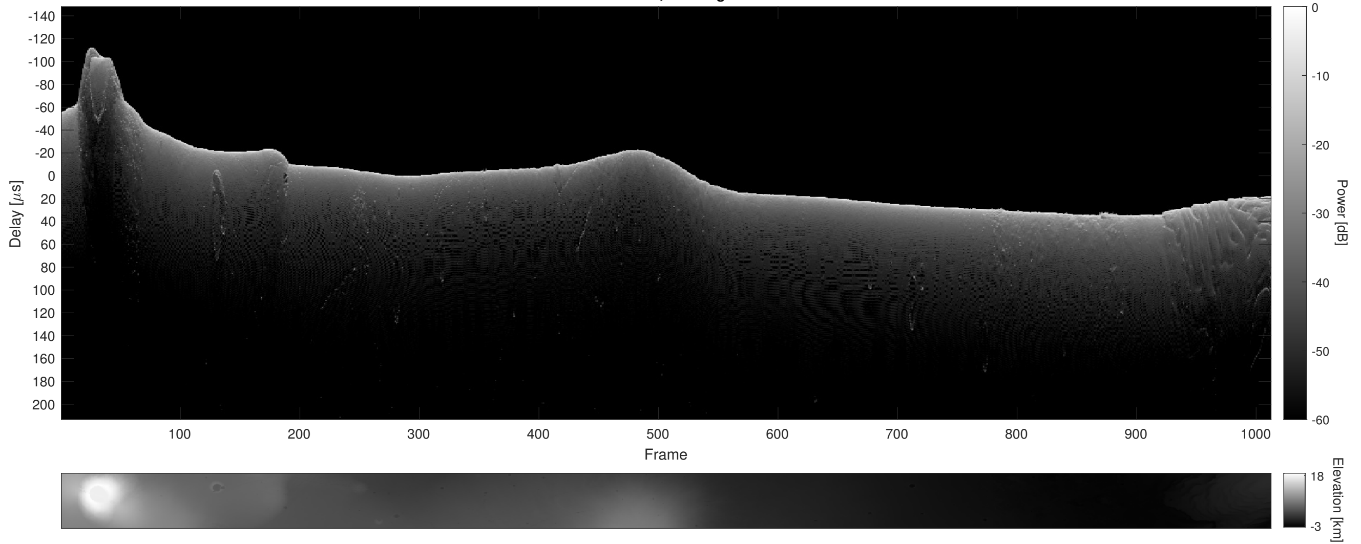
Orbit 10082, Cluttergram
