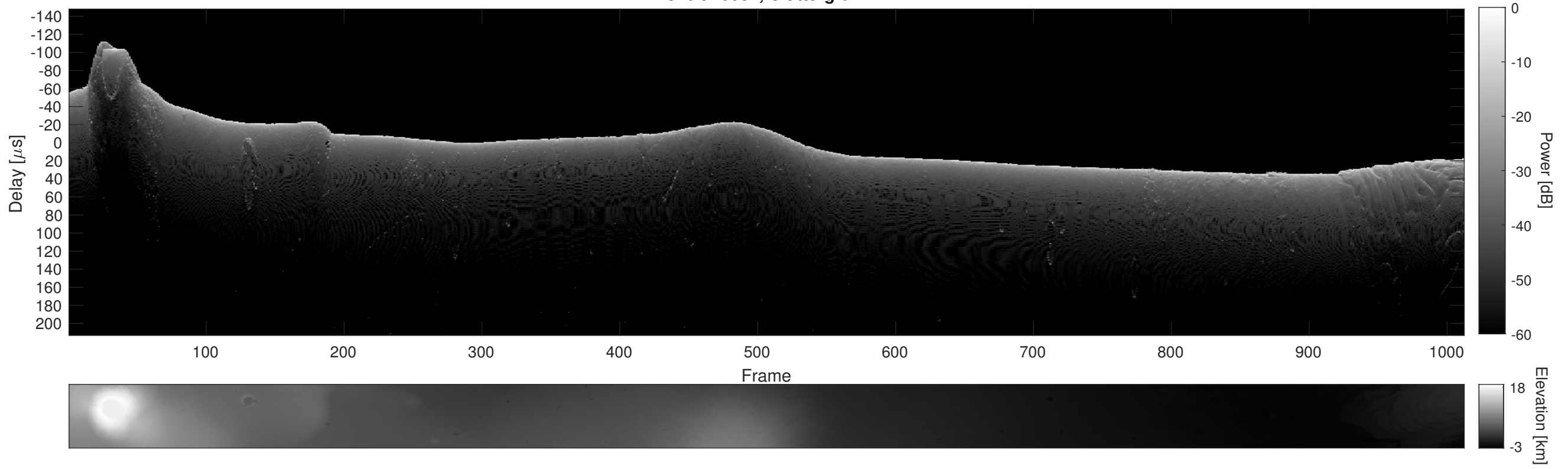
Orbit 10082, Cluttergram
