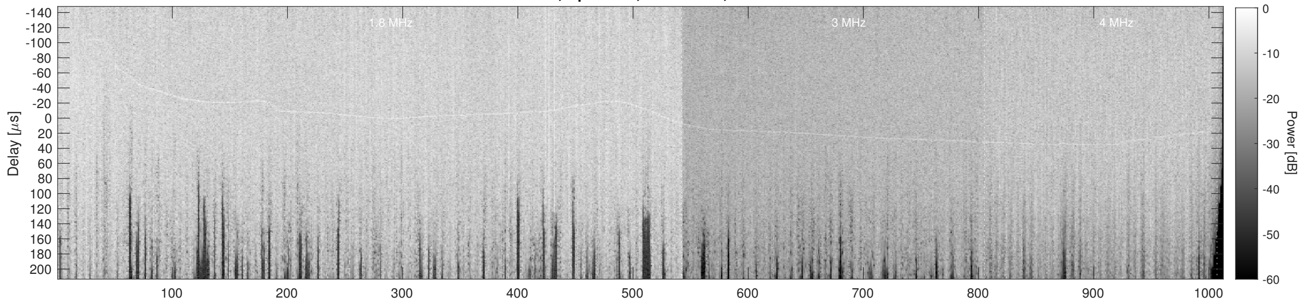
Orbit 10082, Cluttergram
