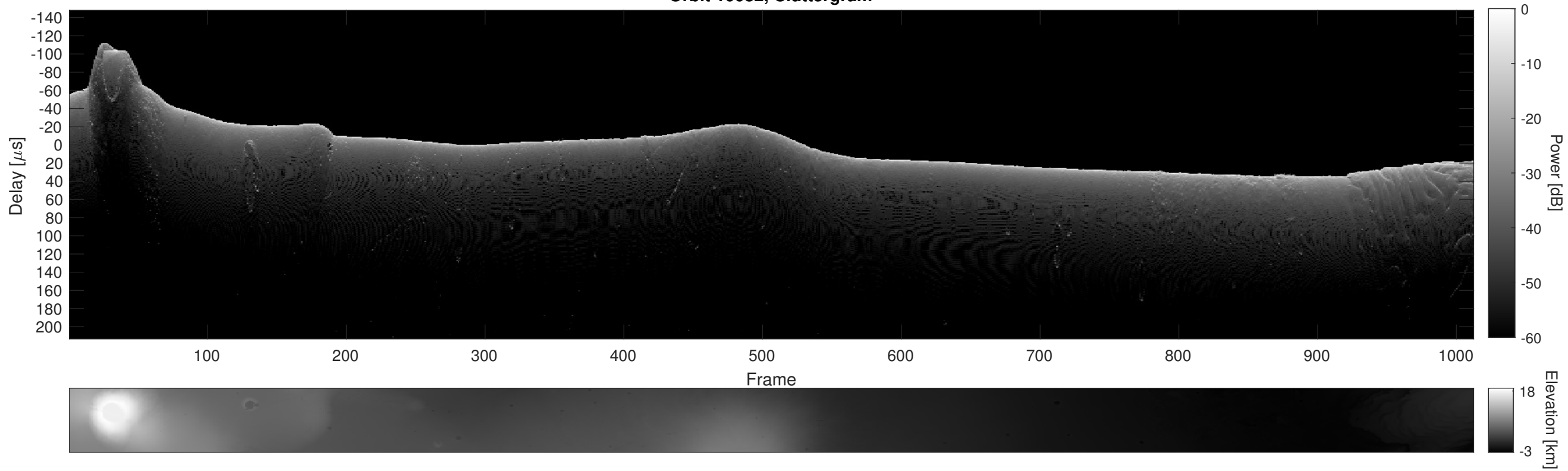
Orbit 10082, Cluttergram
