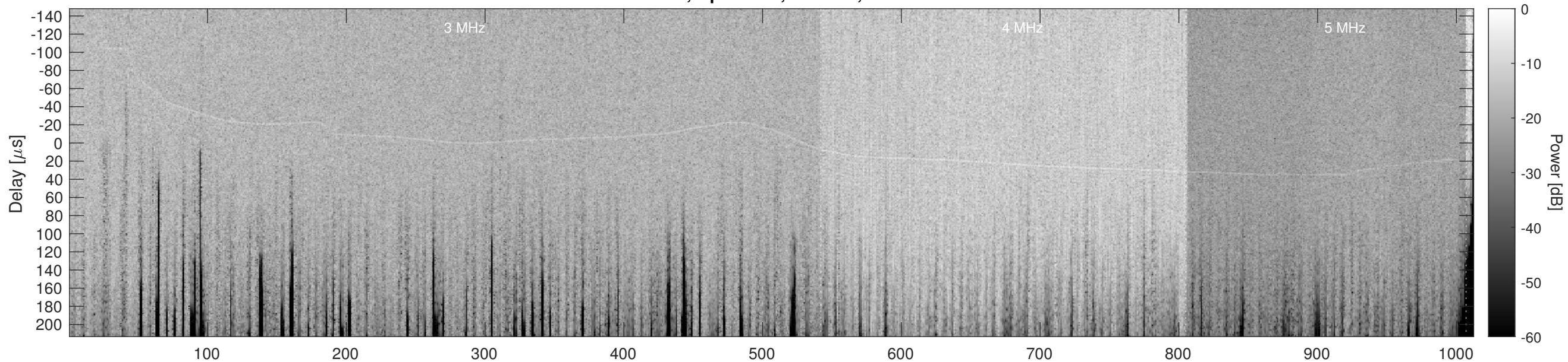
Orbit 10082, Optimized, Window, Channel 2
