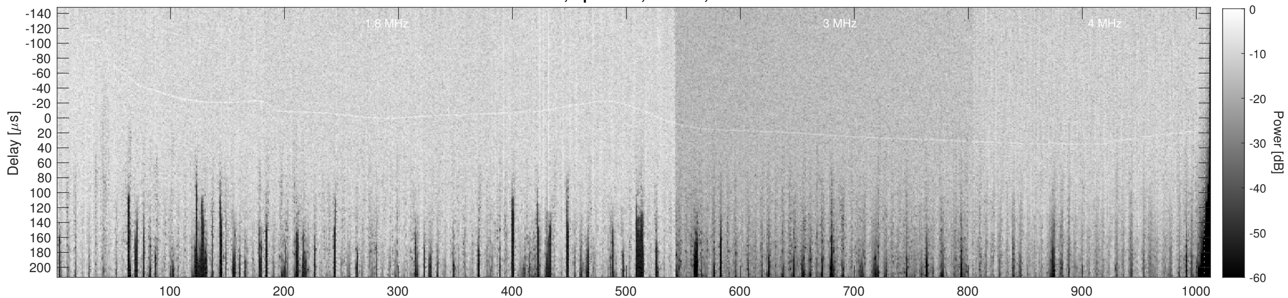
Orbit 10082, Cluttergram
