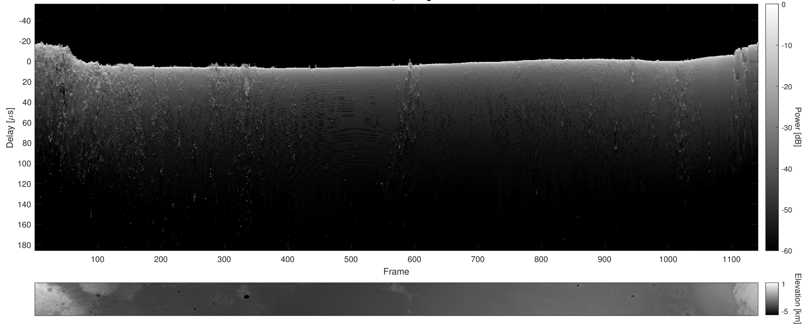
Orbit 10086, Cluttergram
