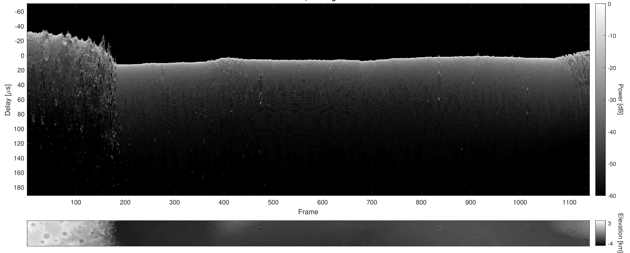
Orbit 10087, Cluttergram
