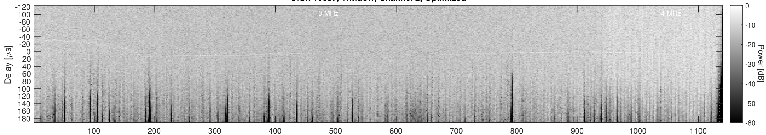
Orbit 10087, Cluttergram
