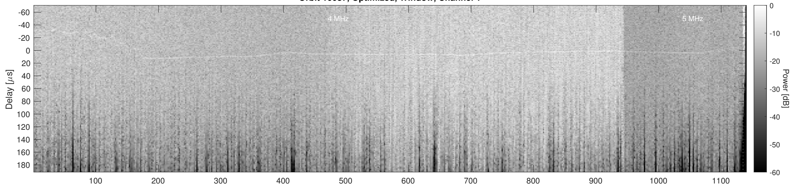
Orbit 10087, Optimized, Window, Channel 2
