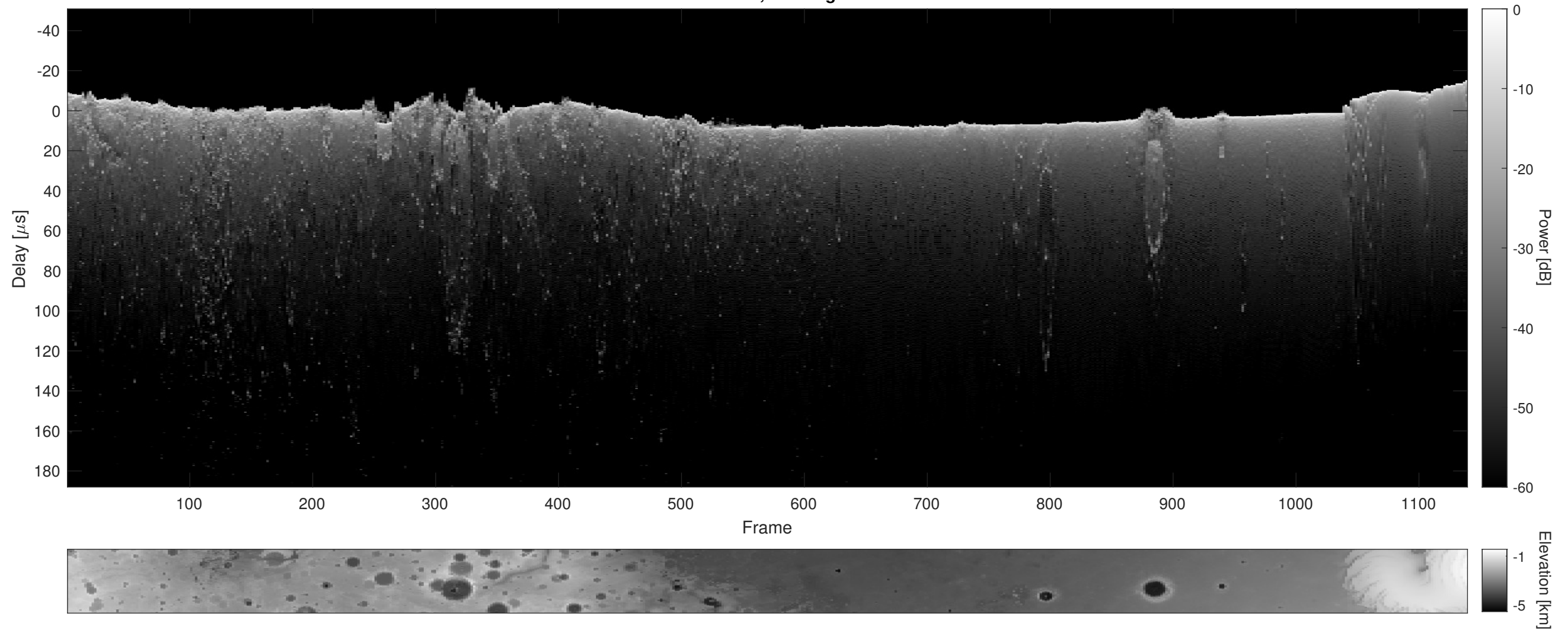
Orbit 10088, Cluttergram
