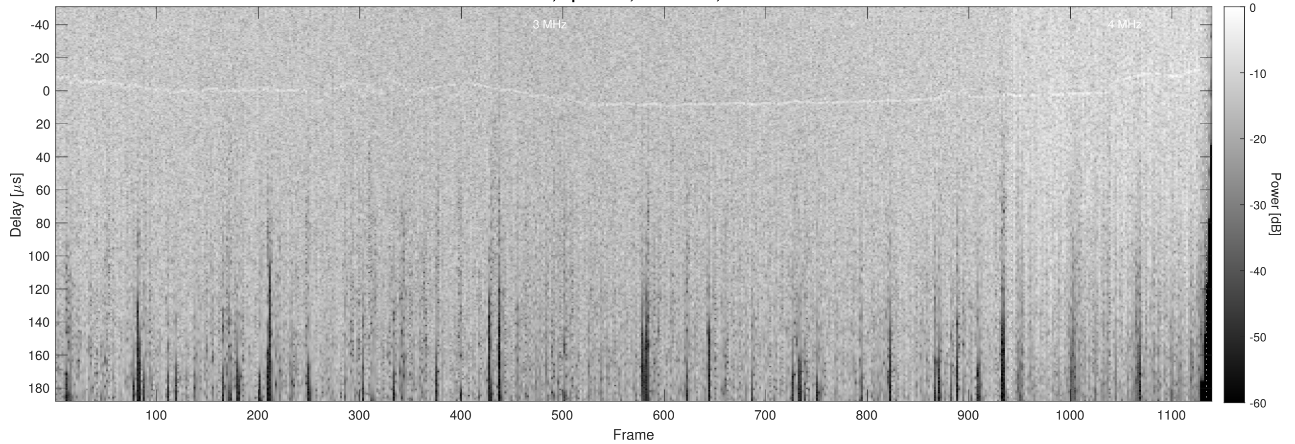
Orbit 10088, Optimized, No Window, Channel 2
