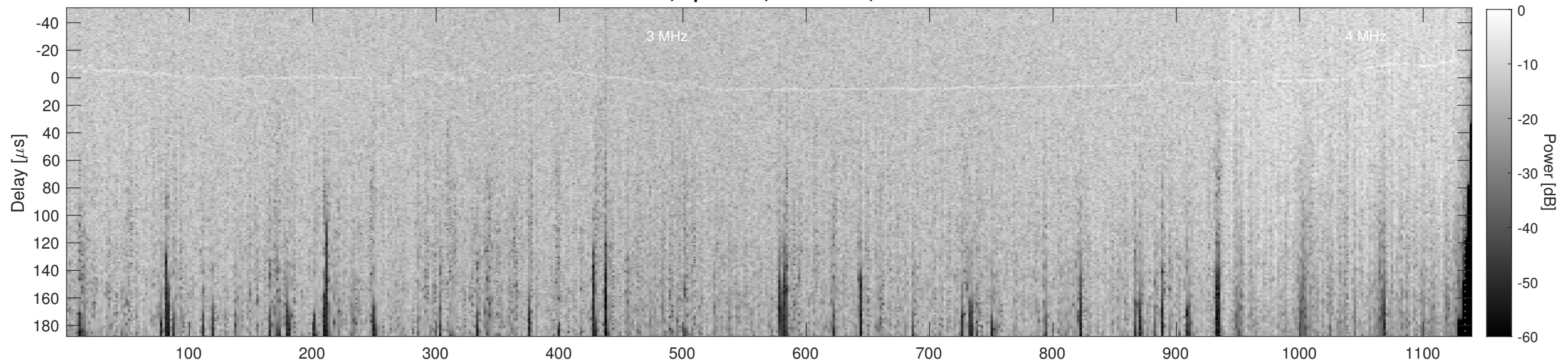
Orbit 10088, Cluttergram
