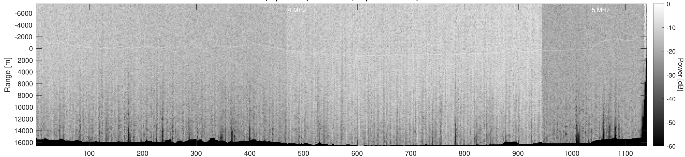
Orbit 10088, Optimized, No Window, Depth-Corrected, Channel 2
