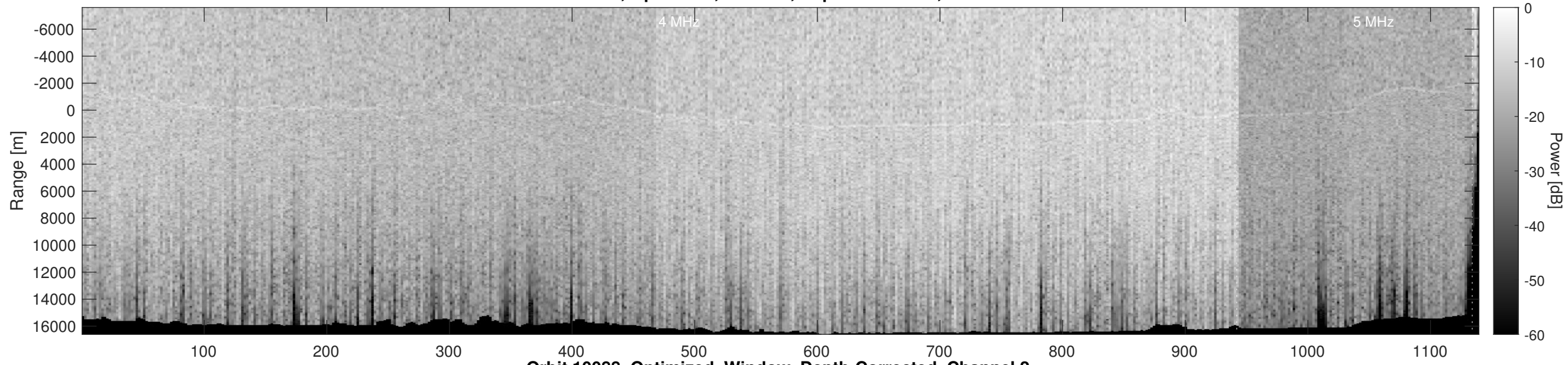
Orbit 10088, Optimized, Window, Depth-Corrected, Channel 2
