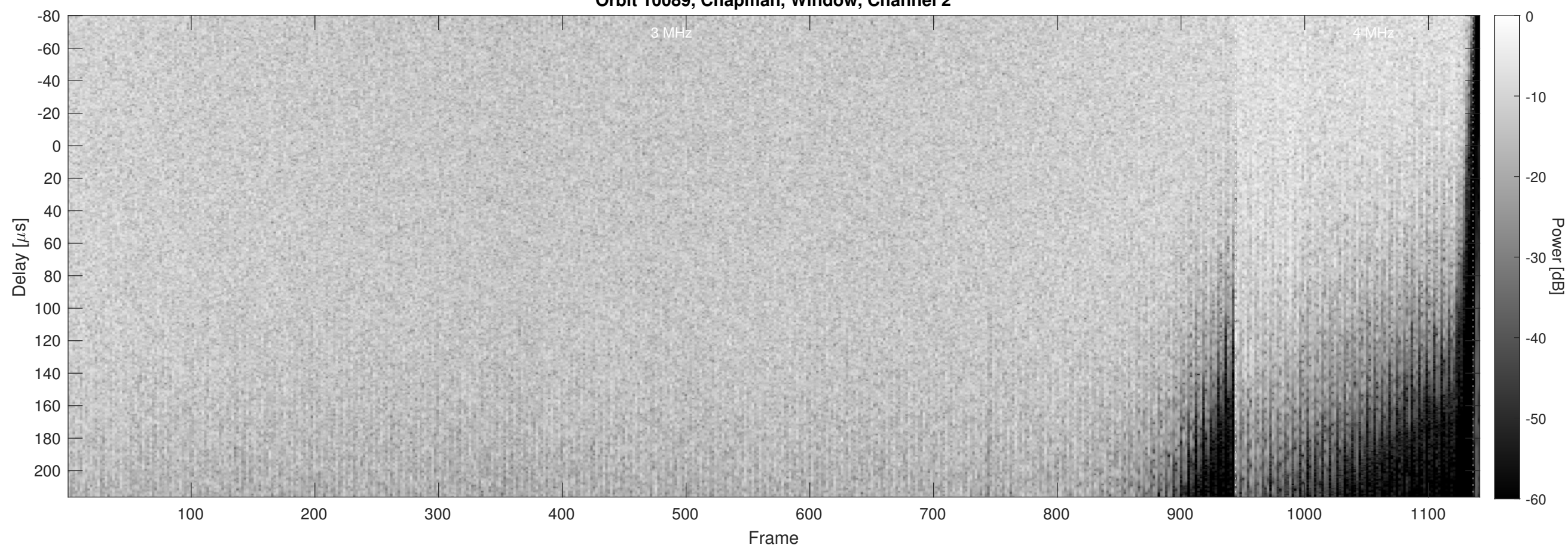
Orbit 10089, Chapman, Window, Channel 2
