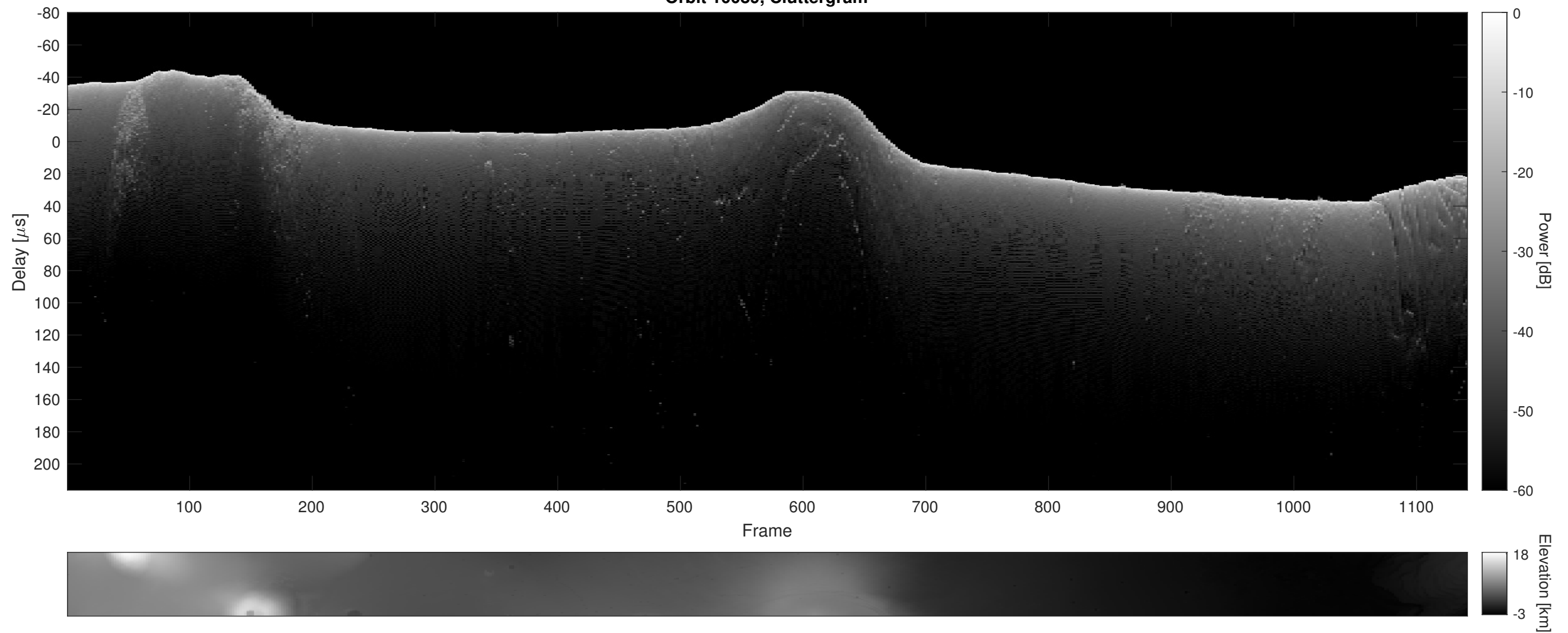
Orbit 10089, Cluttergram
