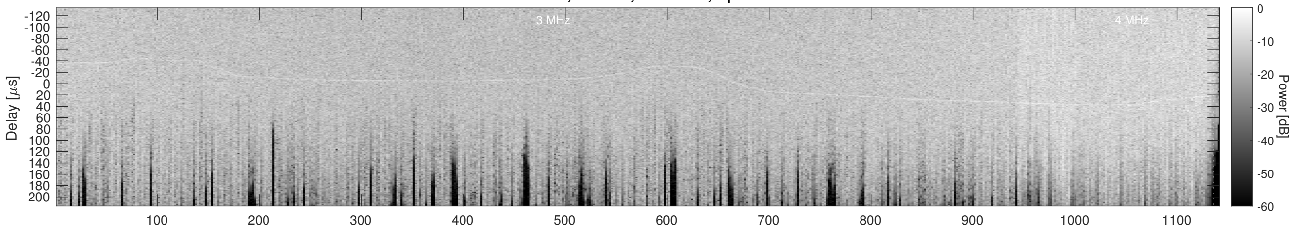
Orbit 10089, Cluttergram
