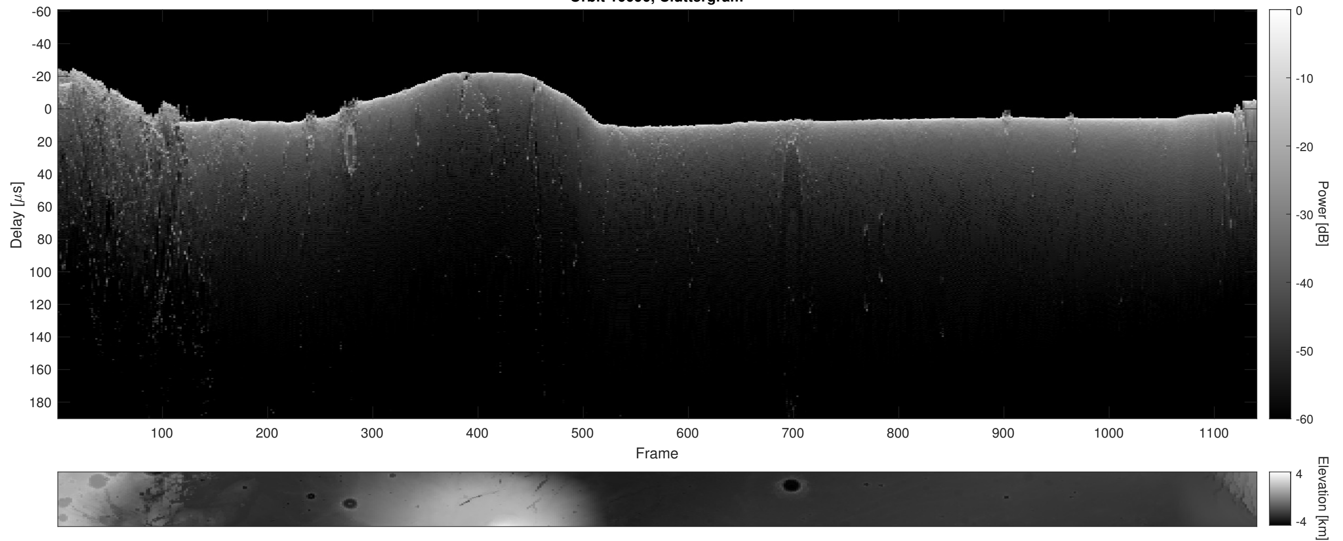
Orbit 10090, Cluttergram
