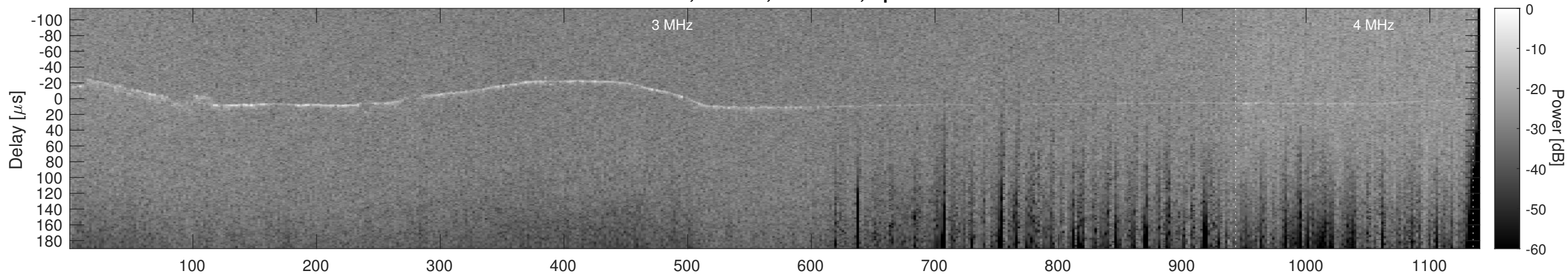
Orbit 10090, Cluttergram
