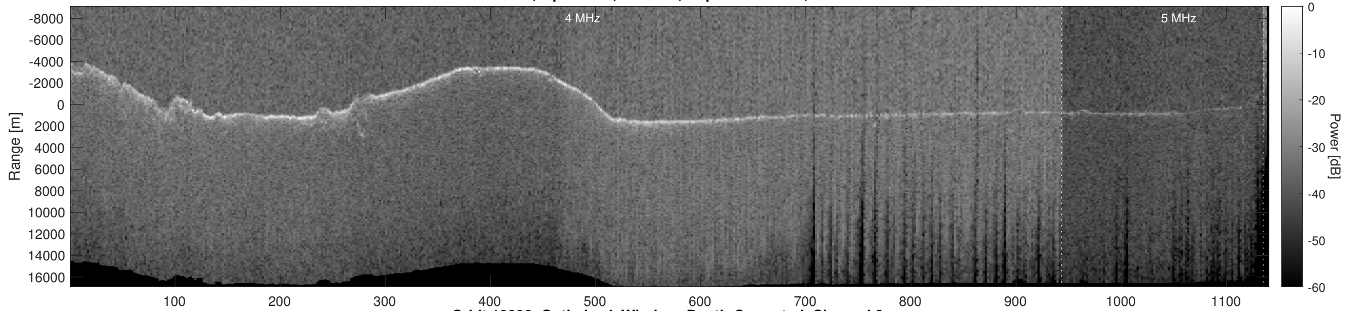
Orbit 10090, Optimized, Window, Depth-Corrected, Channel 2
