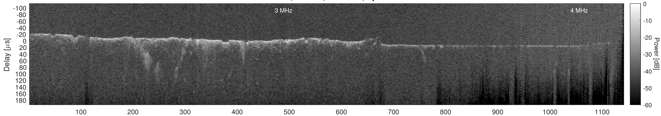
Orbit 10091, Cluttergram
